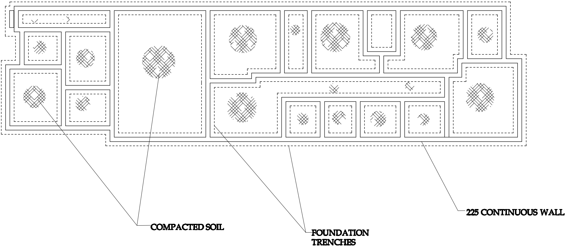
FOUNDATIN PLAN
