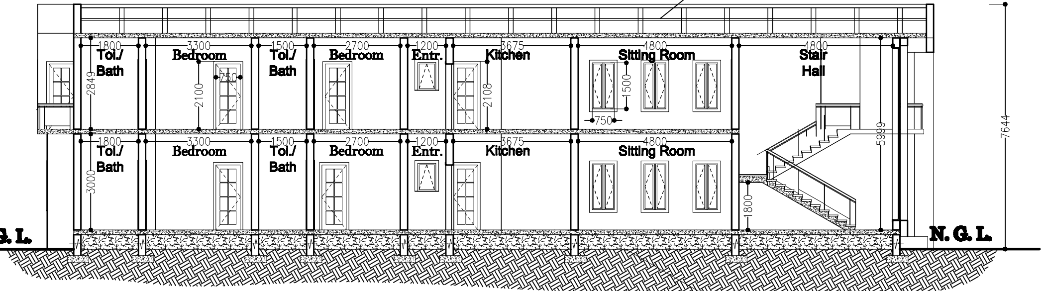
SECTION B-B
